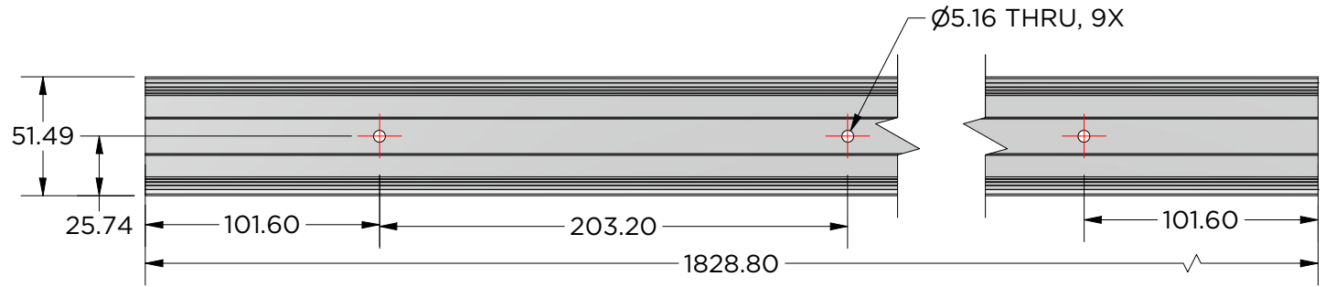
MSNAP-WR72H8 Rail x 1
