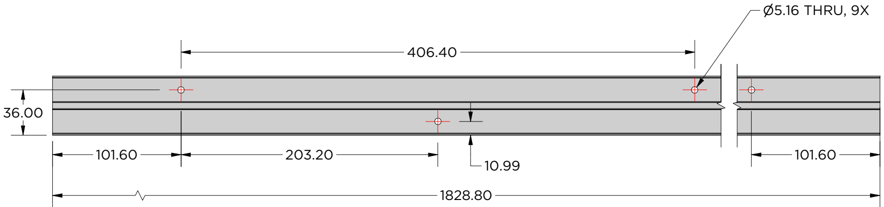
MSNAP-WR72H8 Rail x 1
